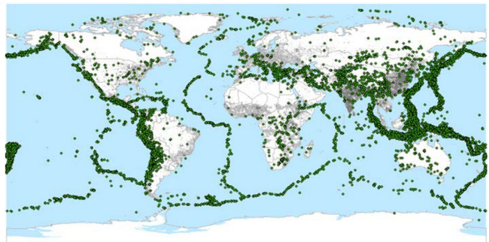
Fig. 1 Epicenters of all earthquakes, September 1968 to June 2008, from PAGER-CAT
